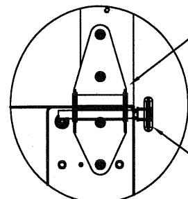
TYPICAL M1000/SUPERFLEX END HINGE N.T.S.
